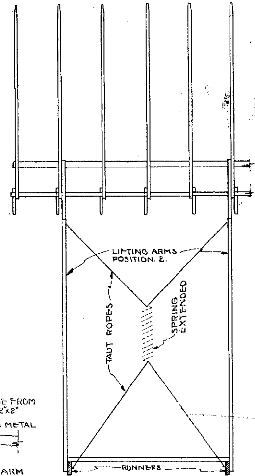
RIGHT END VIEW OF EXTENSION ARMS
