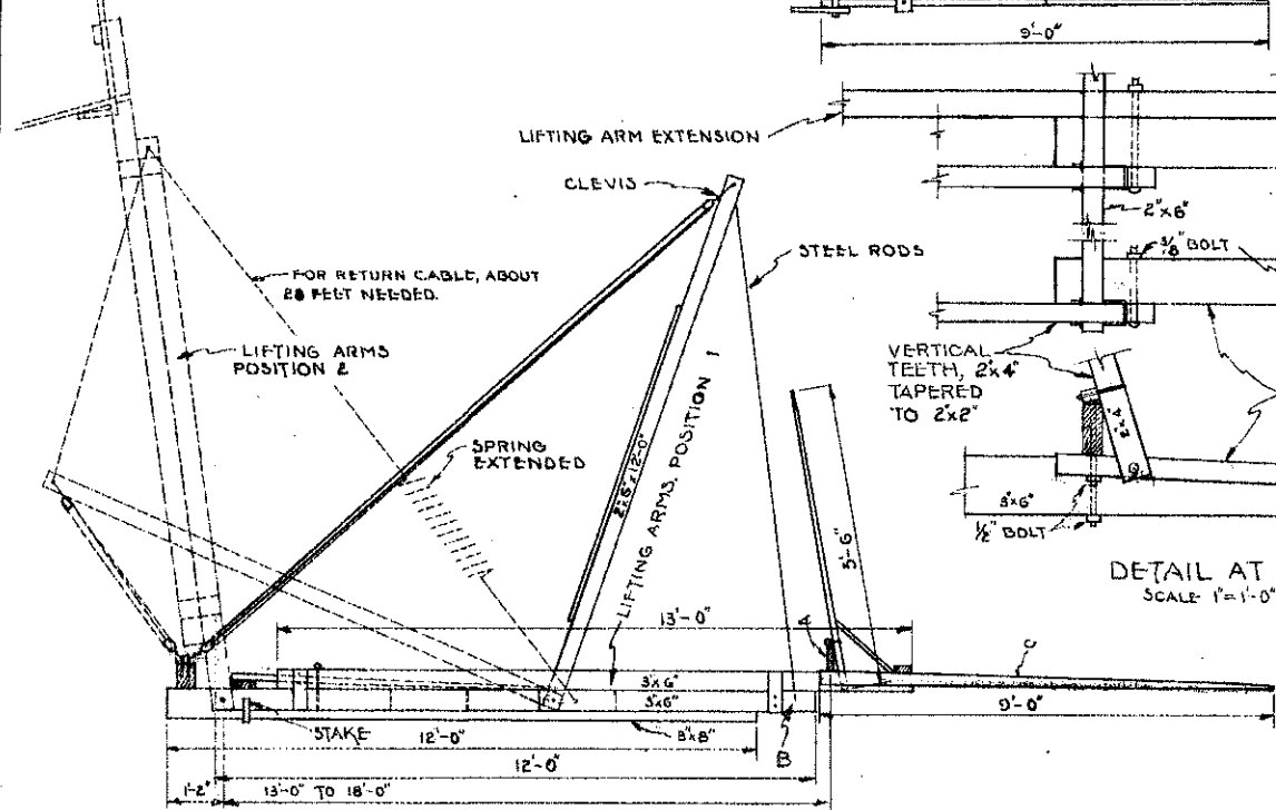
OVERSHOT HAY STACKER SCALE 1/2"=1'-0"
