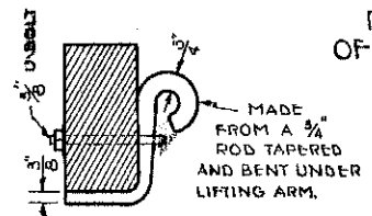
DETAIL AT 'B' STEEL HOOK FOR STEEL ROD
