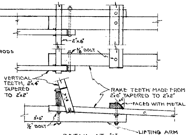
DETAIL AT 'A' SCALE 1"=1'-0"
