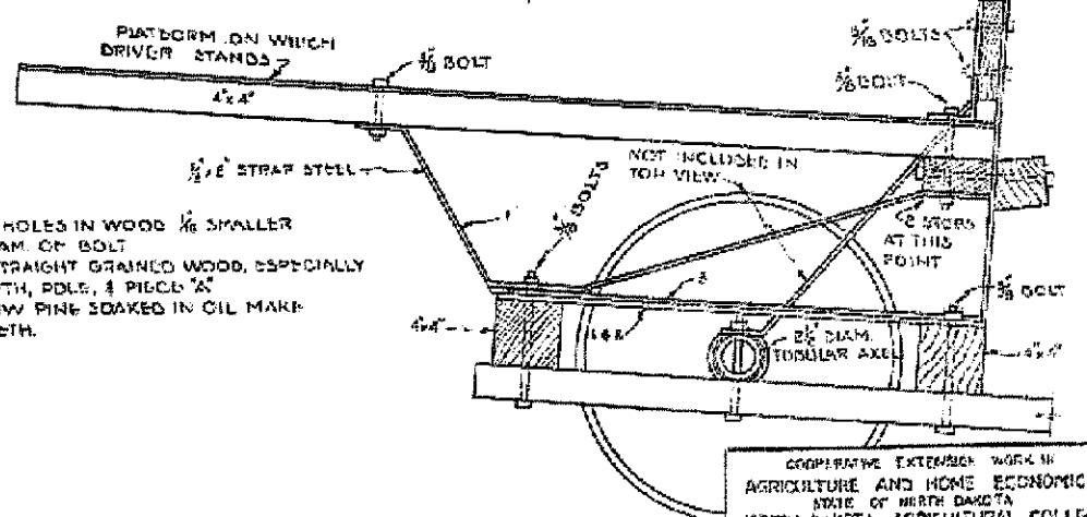
SECTION THRU B-B SCALE 2"-1'-0"
