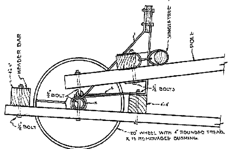
SECTION THRU A-A SCALE 2"-1'-0"
