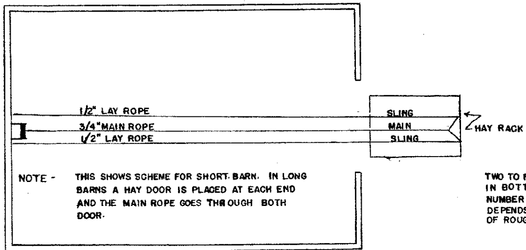
PLAN VIEW OF ROUGHAGE "ROLL-IN"
