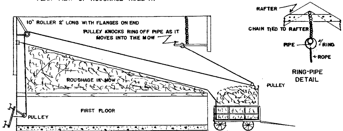
SECTION OF BARN SHOWING ROUGHAGE "ROLL-IN"
