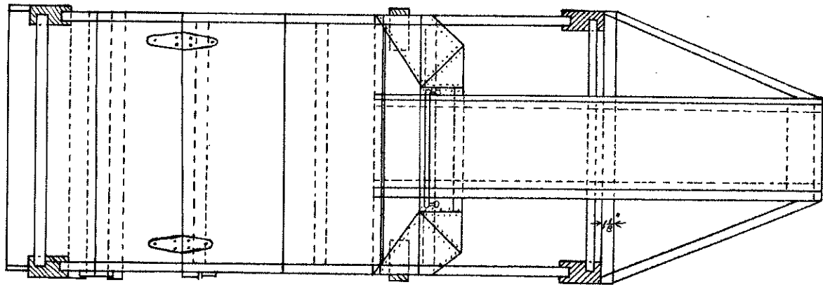
TOP VIEW. Scale 1\frac{1}{2}''=1'
