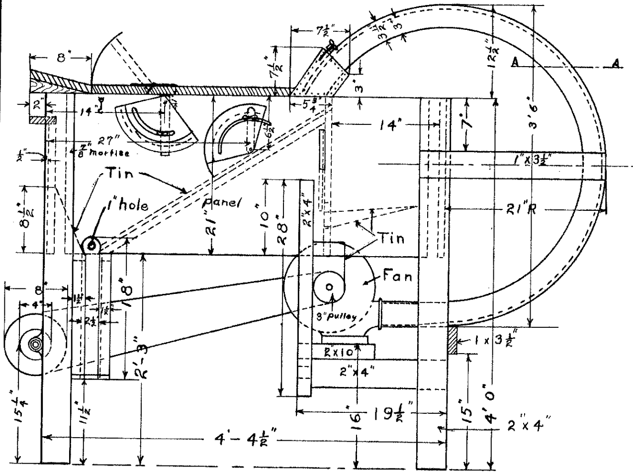
Scale 1\frac{1}{2}''=1' SIDE VIEW.
