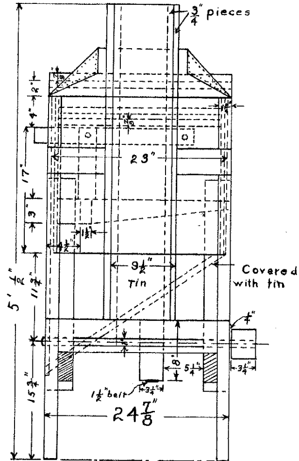
Scale 1\frac{1}{2}''=1' END VIEW.
