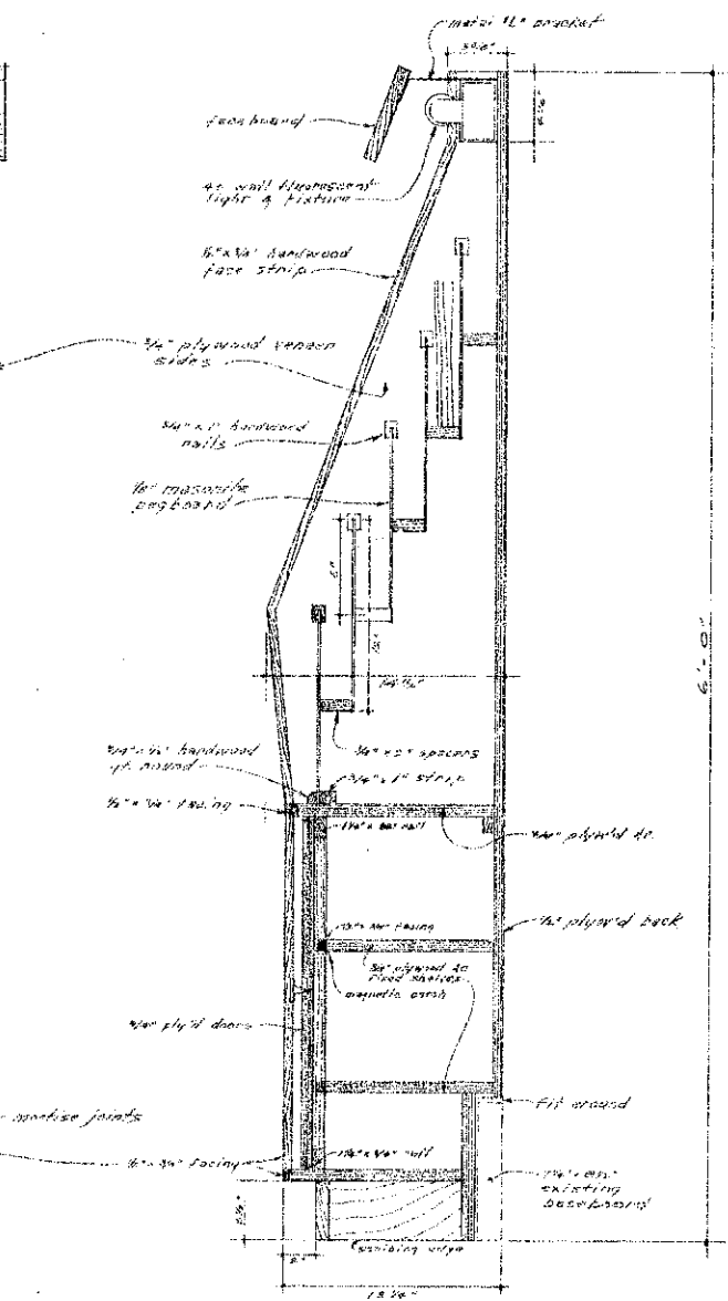
CROSS SECTION VIEW SCALE: 3/8" = 1'-0"
