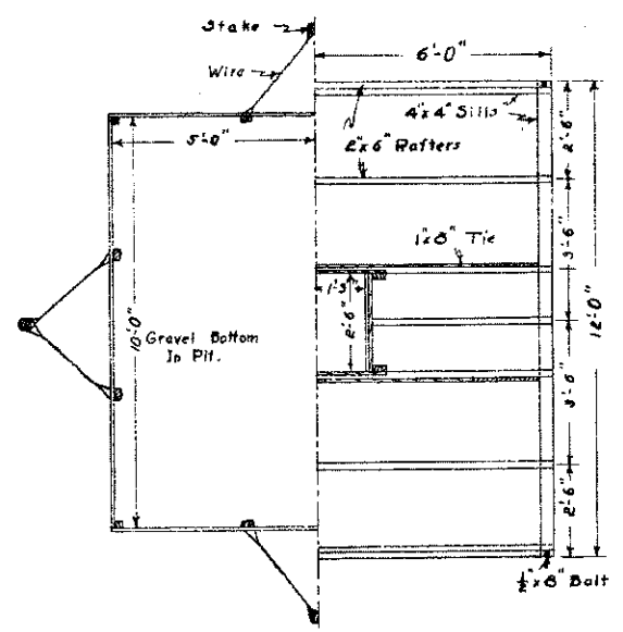
PLAN VIEW Shiplap Retaining Wall Shown on Left, Framing Details of Cover on Right.
