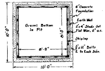
PLAN OF FOUNDATION AND PIT Scale: \frac{1}{4} " = 1'-0"
