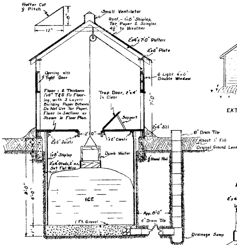
SECTION THROUGH PIT, COVERING AND DRAINAGE SUMP Scale: \frac{3}{8} " = 1'-0"
