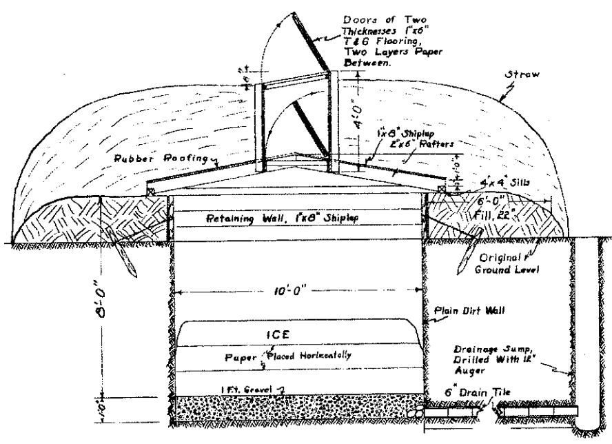
SECTION THROUGH PIT, COVERING AND DRAINAGE SUMP
