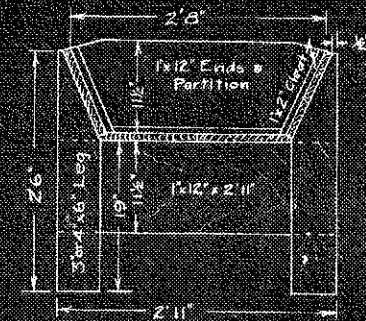
END SECTION
