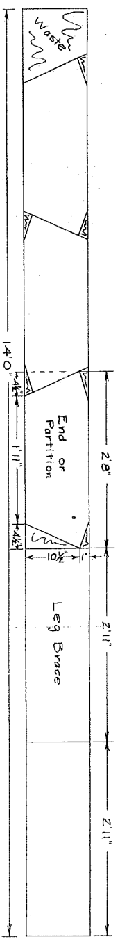
CUTS FOR ENDS, PARTITION, & LEG CROSSPIECES
