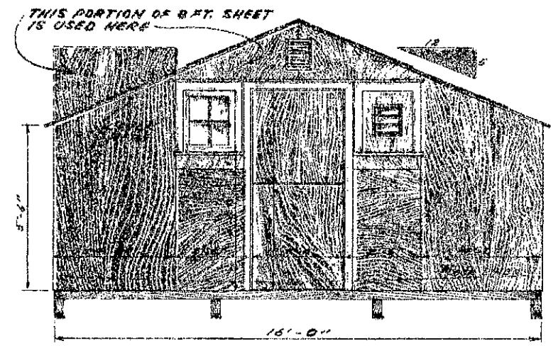
FRONT AND BACK ELEVATION
