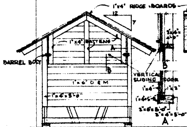
CROSS SECTION SCALE - 3/8" = 1'-0"
