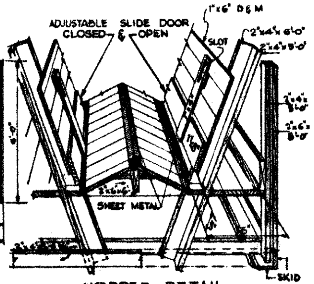
HOPPER DETAIL
