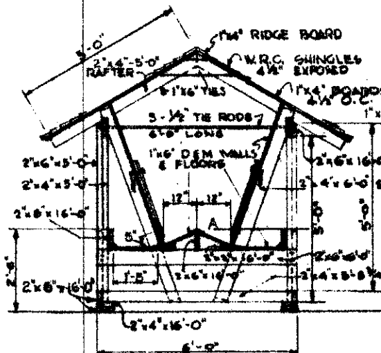
CROSS SECTION SCALE - 3/8" = 1'-0"
