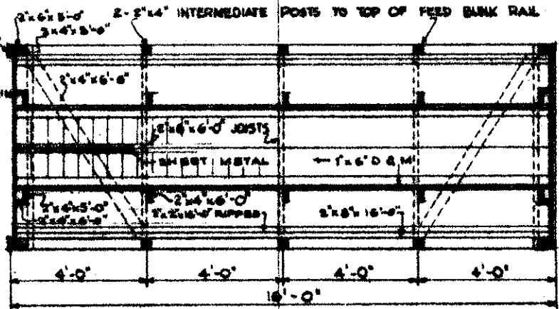
PLAN AT 'A' SCALE 3/8" = 1'-0"
