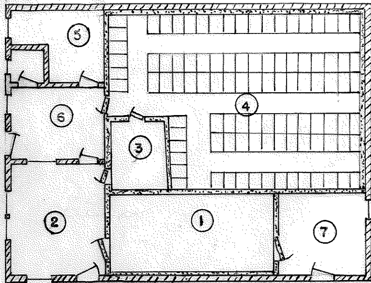
FLOOR PLAN OF A TYPICAL REFRIGERATED LOCKER PLANT
