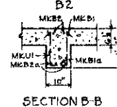
DETAIL OF BEAMS B1 & B2 SCALE 1/2" = 1'-0"
