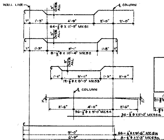
VENT SHAFT BARS
