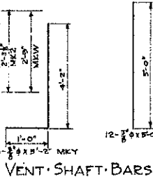
VENT SHAFT BARS
