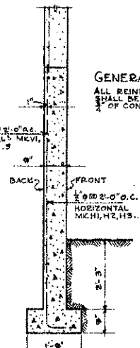
SECTION THRU RETAINING WALL SCALE 1/2" = 1'-0"
