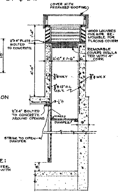
VERTICAL SECTION THRU VENTILATION INTAKE SHAFT SCALE 1/2" = 1'-0"
