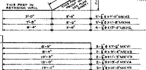
RETAINING WALL BARS
