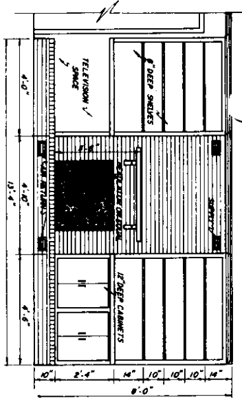
ELEVATION A SCALE 1/2" = 6'-0"
