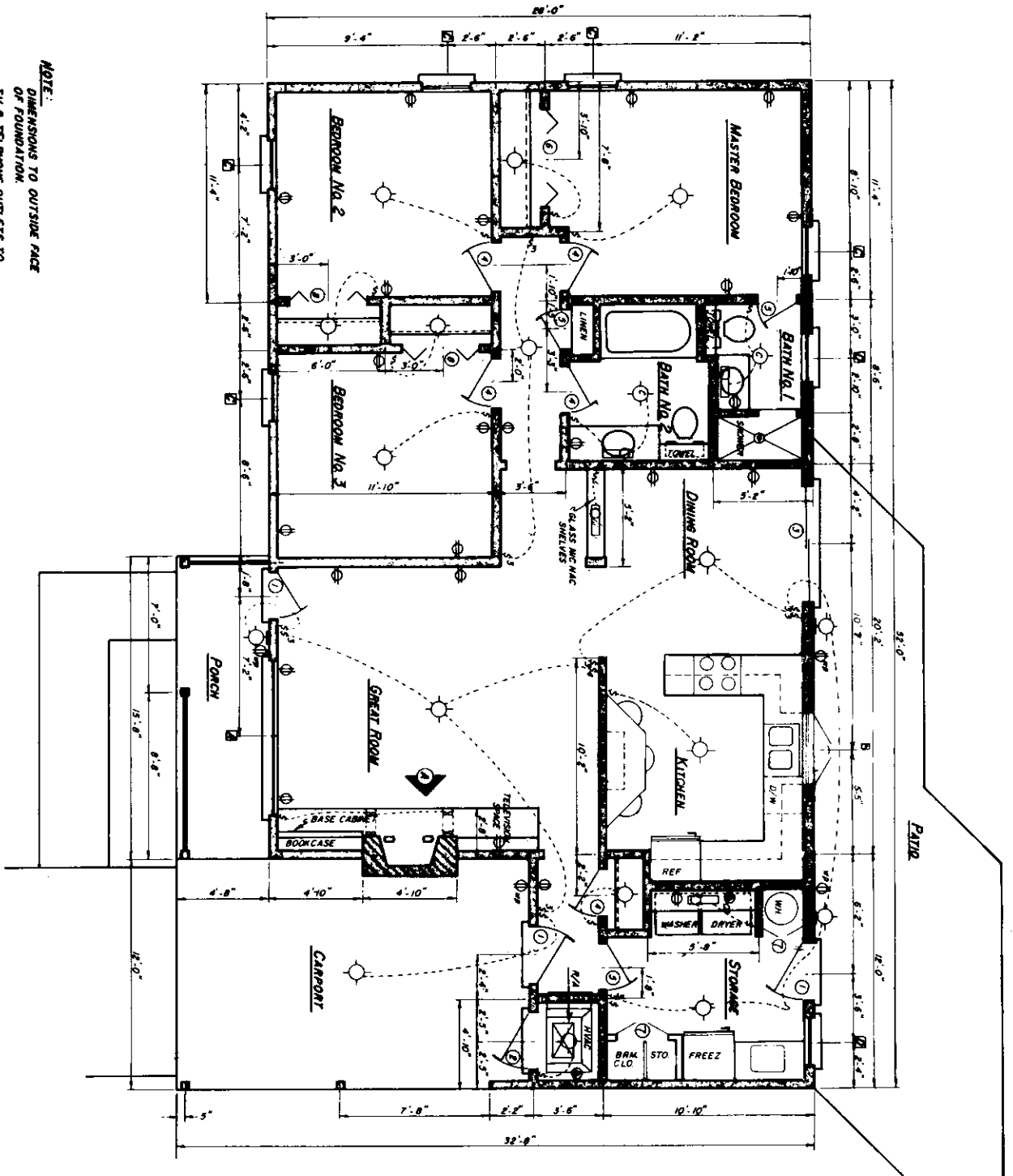
FLOOR PLAN
