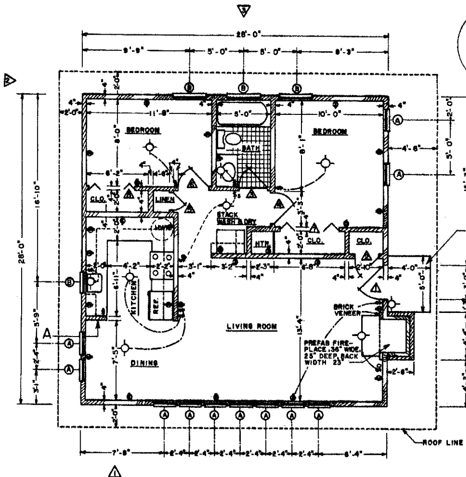
FLOOR PLAN SCALE: 1/4" = 1'-0" 0' 2' 4' 6'
