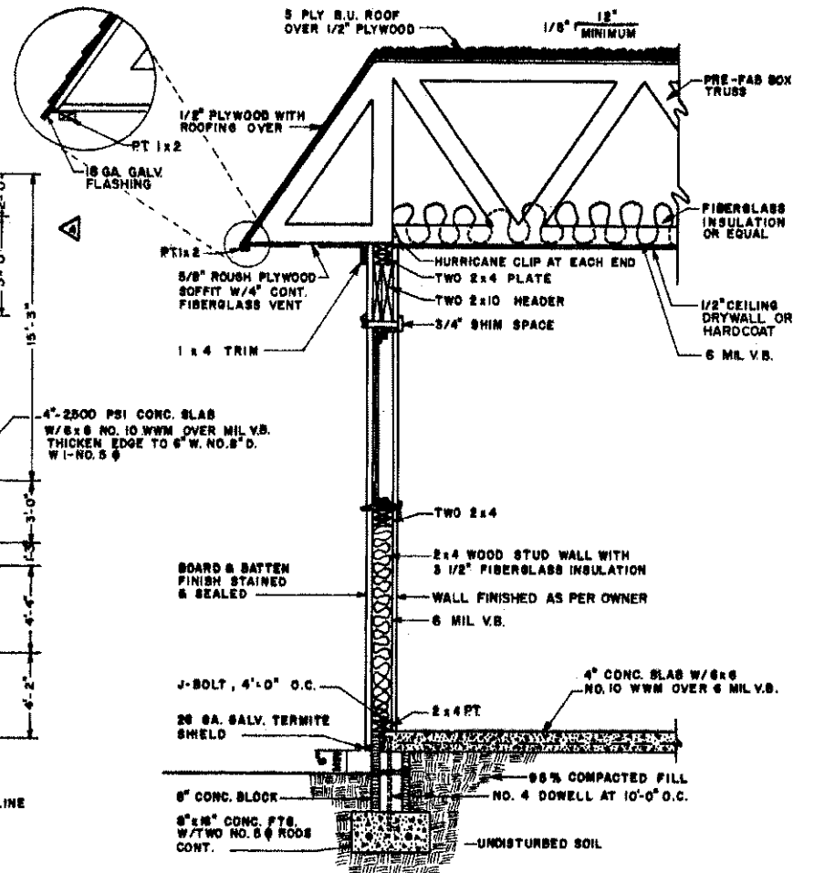
TYPICAL WALL SECTION SCALE: 3/4" = 1'-0" 0' 2' 4' 6'
