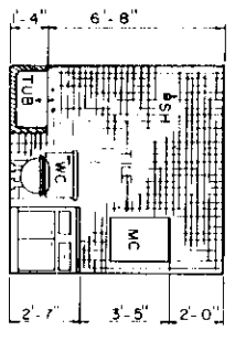
DETAIL-1
