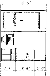
DETAIL-4
