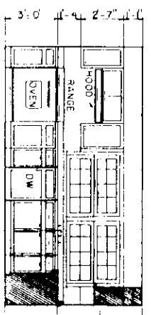
DETAIL-2
