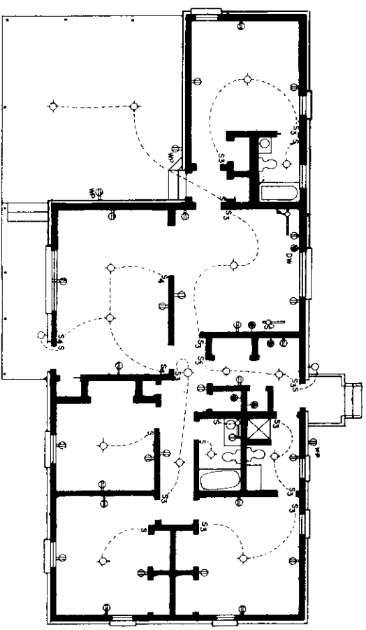
ELECTRICAL PLAN
