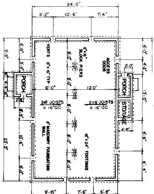
FOUNDATION PLAN
