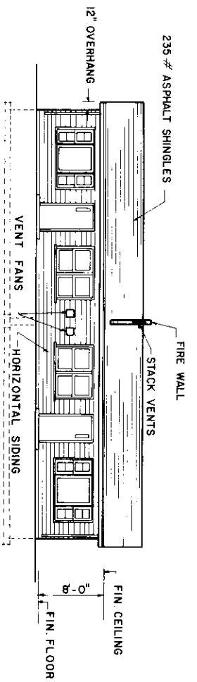
FRONT ELEVATION
