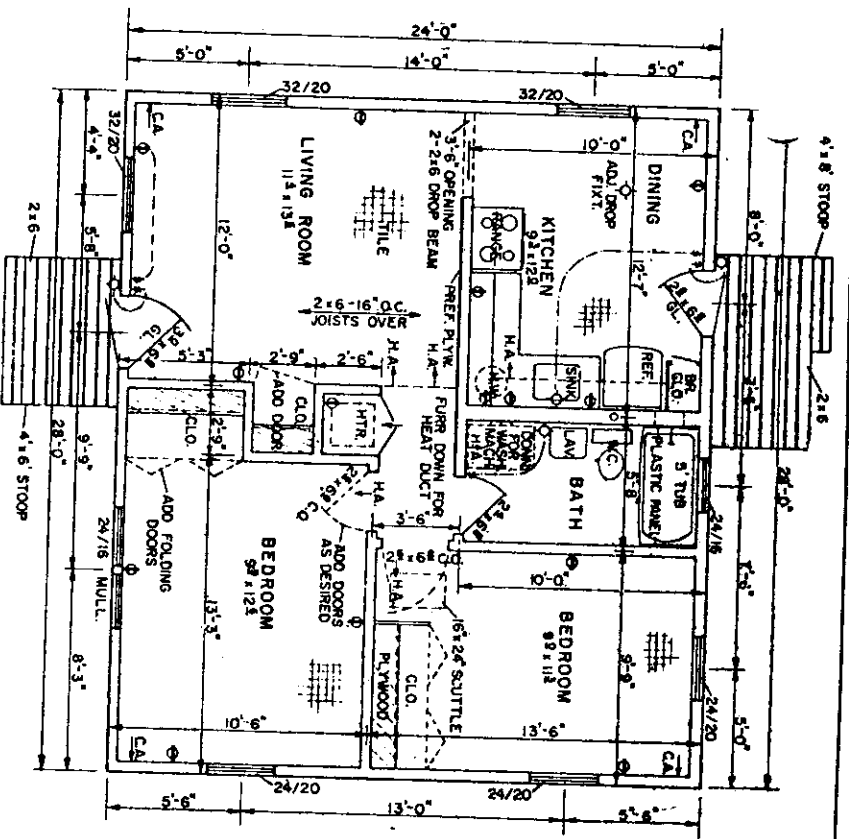
FLOOR PLAN ONE STORY DESIGN (A)
