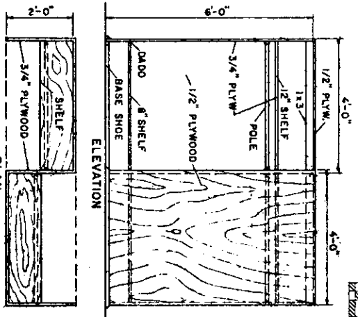
WARDROBE EXPANDABLE DESIGN C
