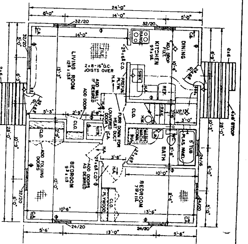
FIRST FLOOR PLAN EXPANDABLE DESIGN (B) (SEE SHEET 5 FOR SECOND FLOOR PLAN)
