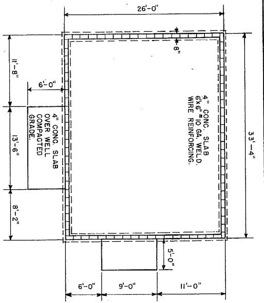
FOUNDATION PLAN SCALE 1/8" = 1'-0"
