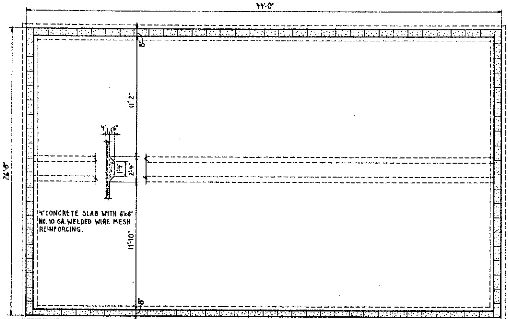
FOUNDATION PLAN SCALE 1/4" = 1'-0"
