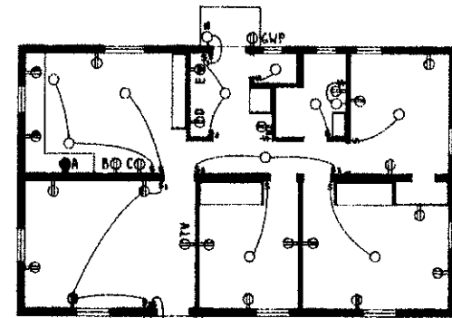
ELECTRICAL LAYOUT
