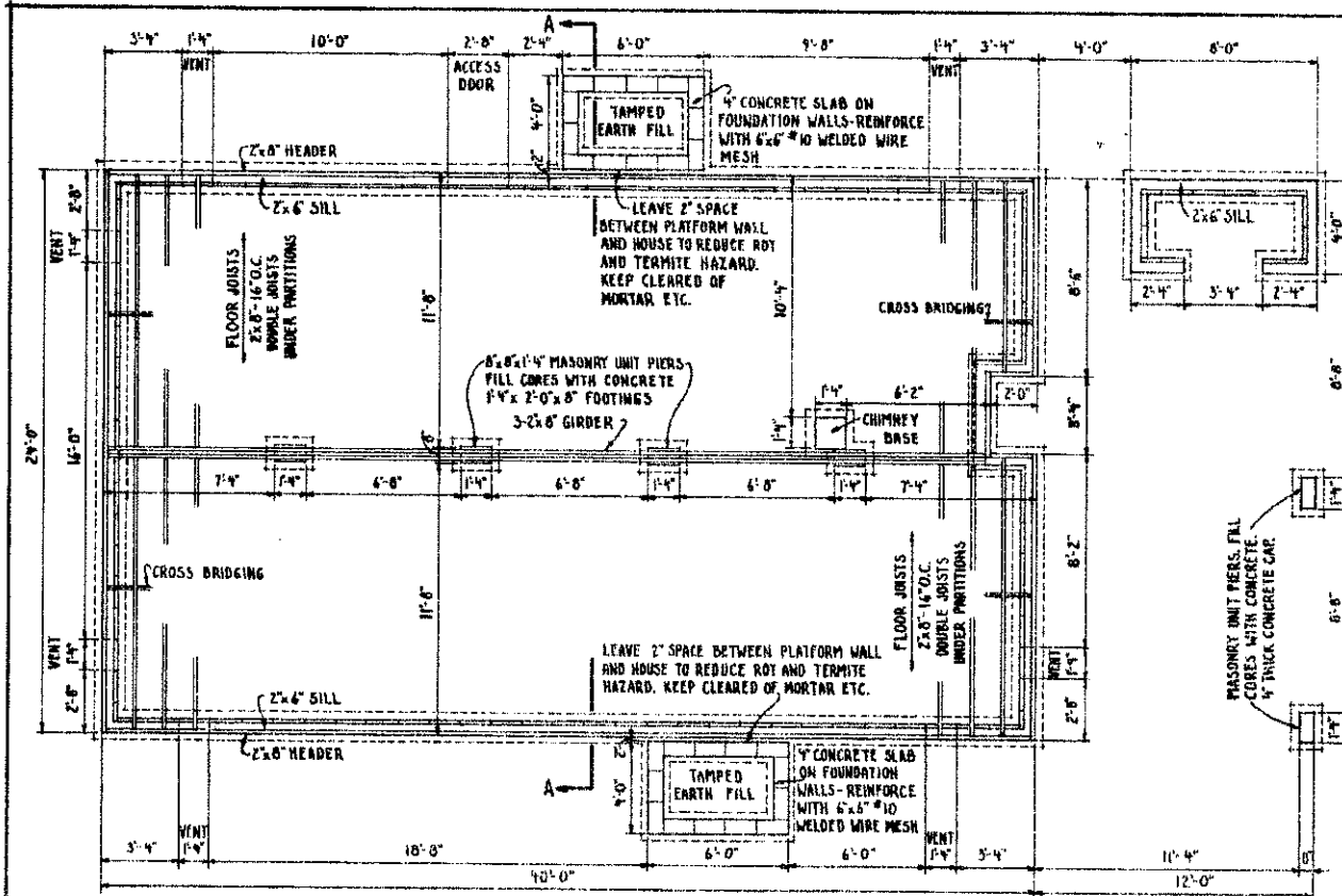
FOUNDATION PLAN SCALE 3/8"=1'-0" DIMENSIONS ARE SHOWN TO FACE OF MASONRY
