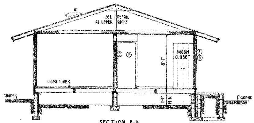
SECTION A-A SCALE 3/8"=1'-0"
