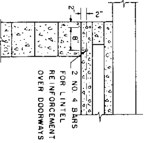
SECTION B-B SCALE 0 2 FT
