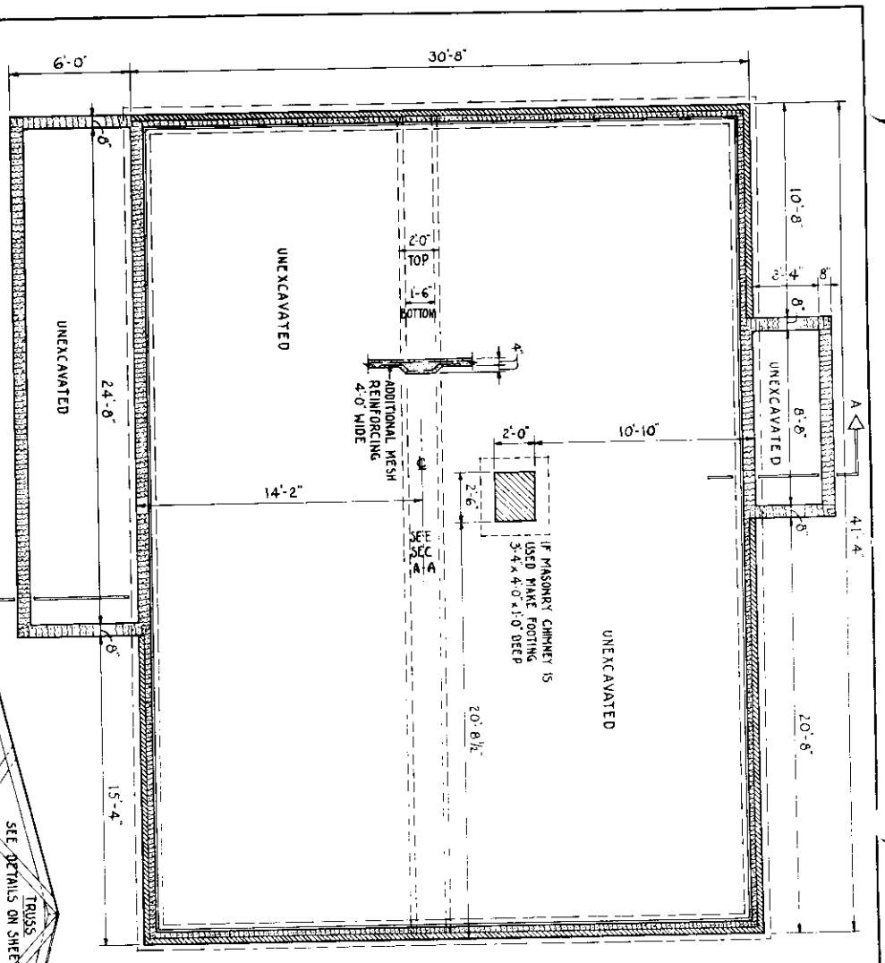
FOUNDATION PLAN
