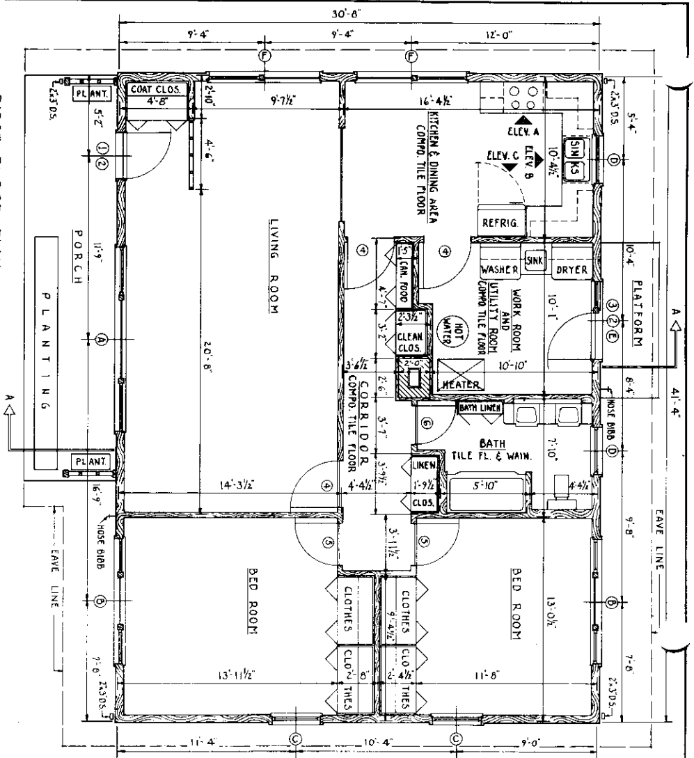
FIRST-FLOOR-PLAN
