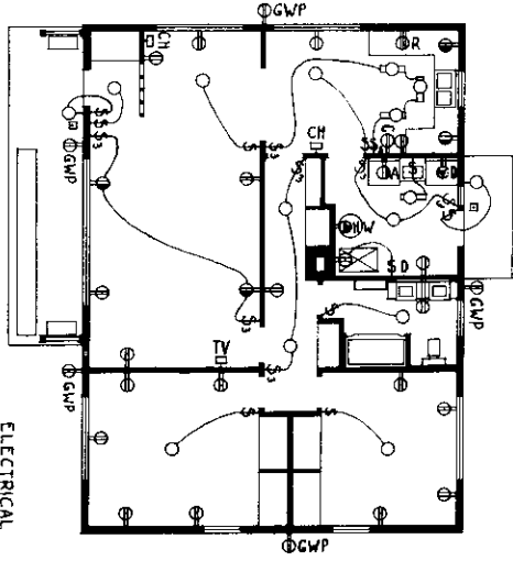
ELECTRICAL LAYOUT
