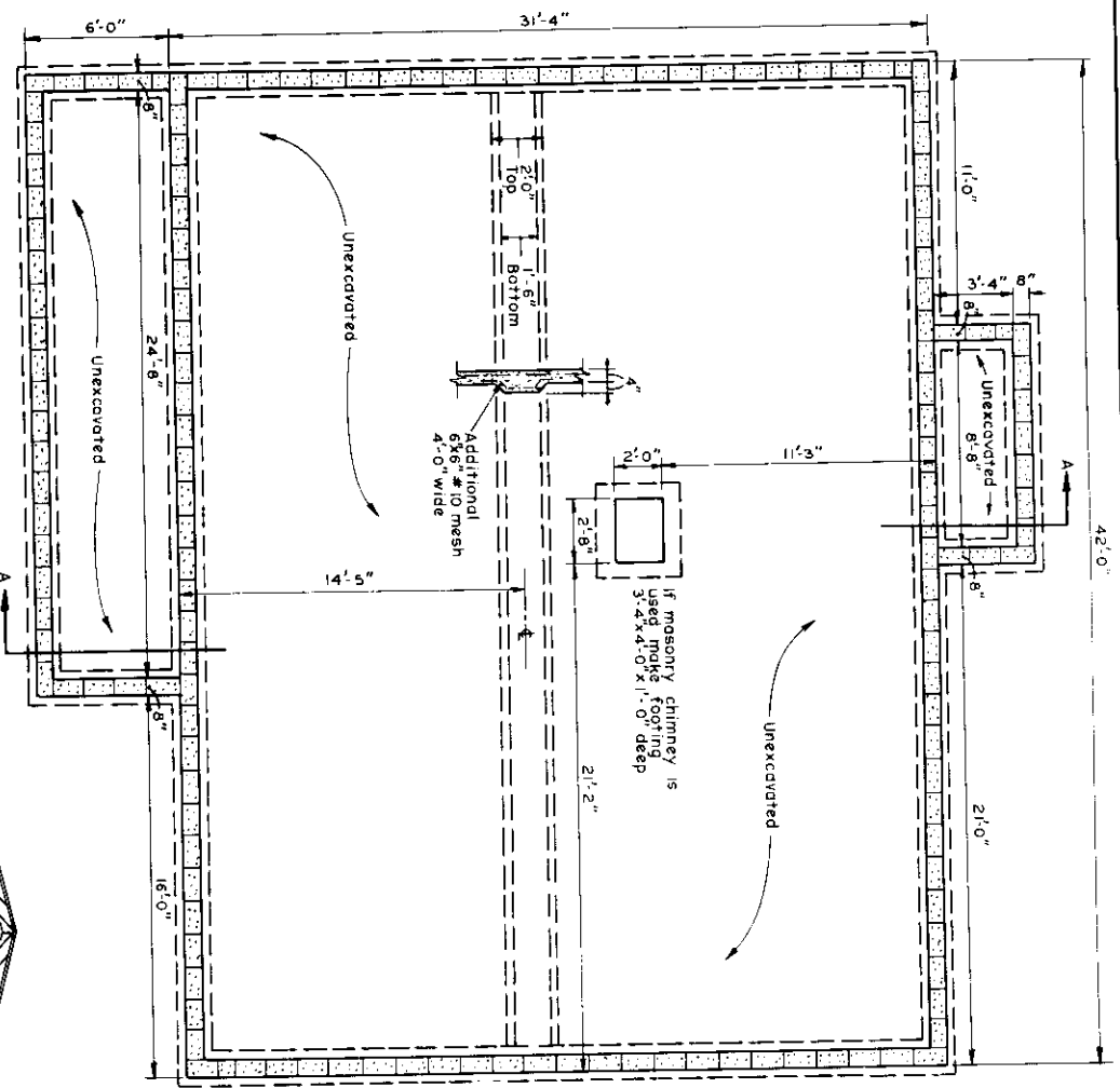
FOUNDATION PLAN
