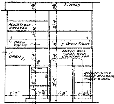
KITCHEN CABINET ELEVATION B
