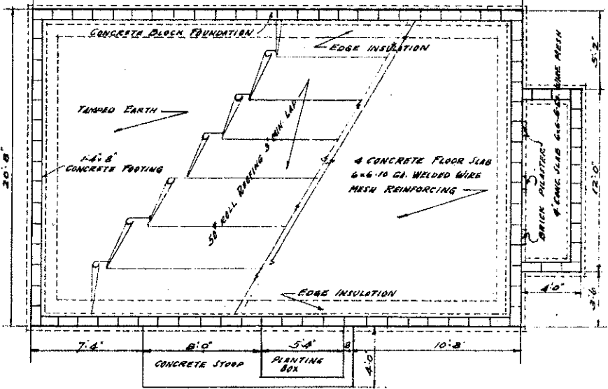
FOUNDATION PLAN SCALE 1/4" = 1'-0"
