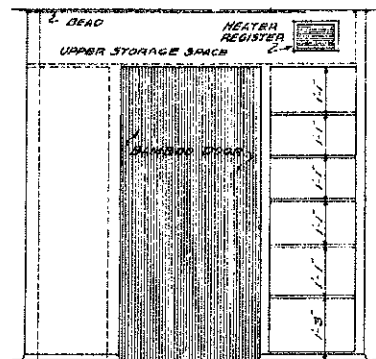
CLOSET UNIT ELEVATION 2
