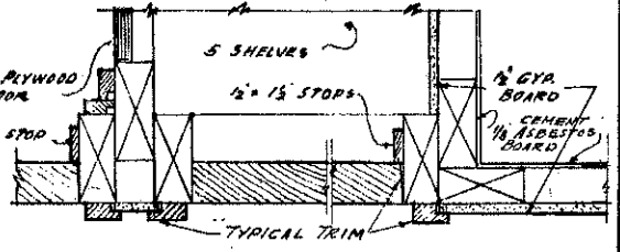
LINEN CLOSET SCALE 3"=1'-0"
