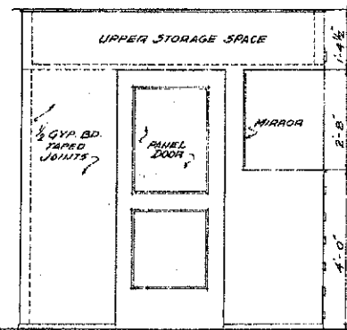
CLOSET UNIT ELEVATION 3
