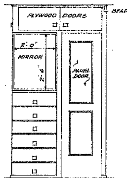
CLOSET UNIT ELEVATION 1
