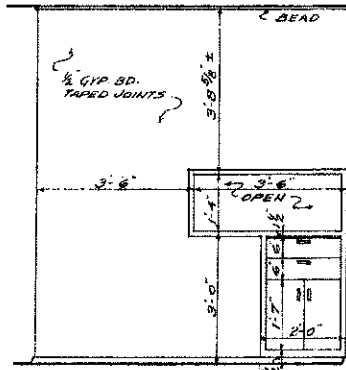
KITCHEN CABINET ELEVATION A
