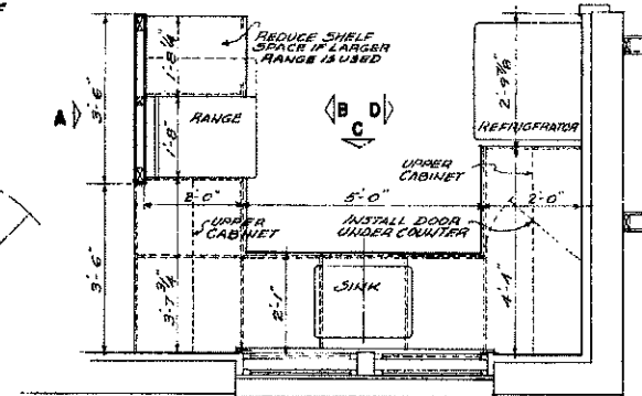
PLAN OF KITCHEN CABINETS
