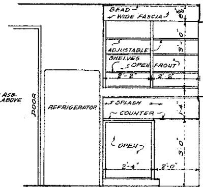
KITCHEN CABINET ELEVATION D
