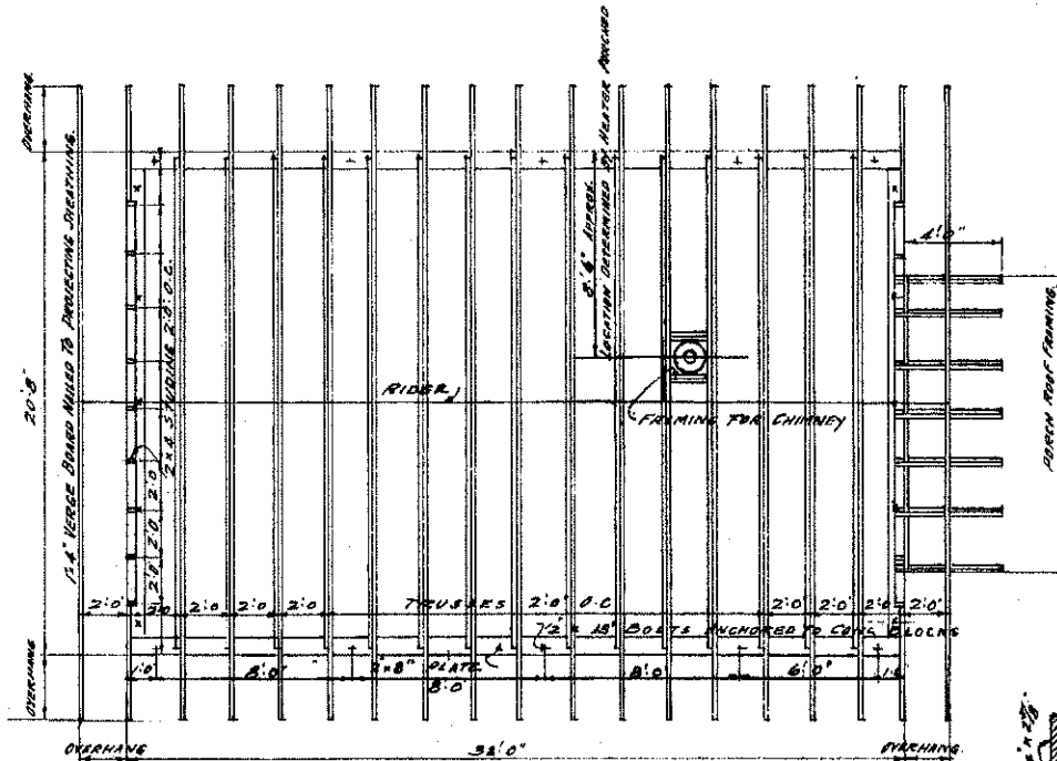
ROOF FRAMING PLAN SCALE 1/4"=1'-0"
