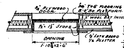
ATTIC SCUTTLE SCALE 1"=1'-0"
