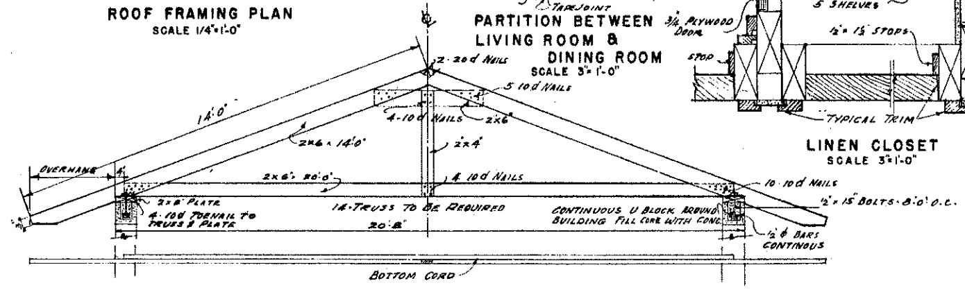
TYPICAL ROOF TRUSS SCALE 1/2"=1'-0"
