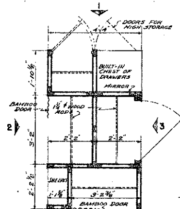
PLAN OF CLOSET UNIT
