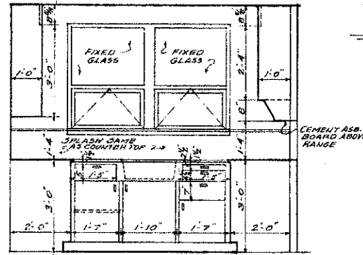
KITCHEN CABINET ELEVATION C
