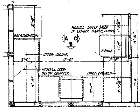
PLAN OF KITCHEN CABINETS
