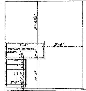
KITCHEN CABINET ELEVATION D
