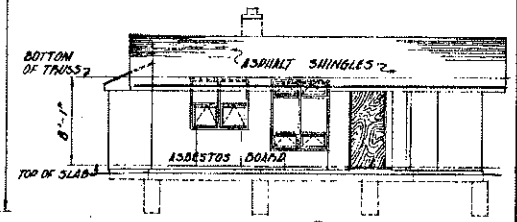
ELEVATION D
