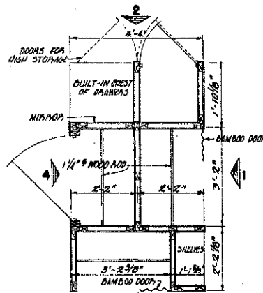
PLAN OF CLOSET UNIT
