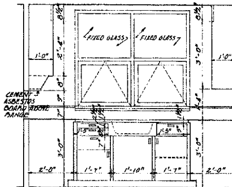
KITCHEN CABINET ELEVATION B
