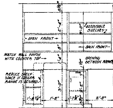
KITCHEN CABINET ELEVATION C
