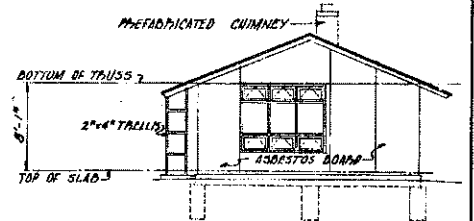
ELEVATION C
