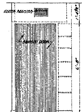
CLOSET UNIT ELEVATION 3
