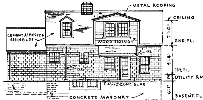
REAR ELEVATION
