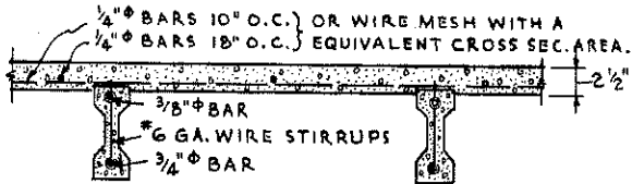
DETAIL OF SLAB REINFORCEMENT
