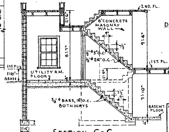
SECTION C-C SHEET-1
