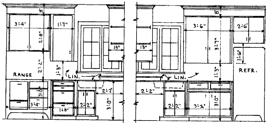
KITCHEN CABINETS SCALE \frac{1}{2}'' = 1'-0''
