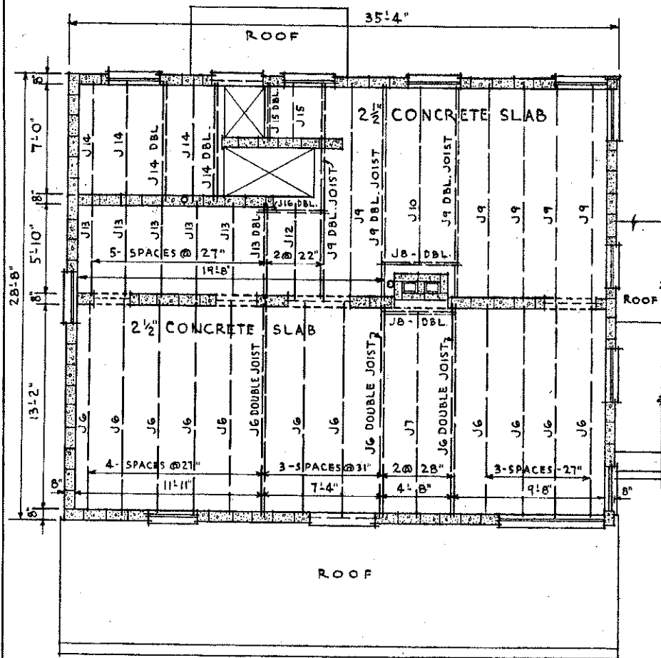
FRAMING FOR SECOND FLOOR CONCRETE JOISTS
