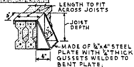
HANGER DETAIL
