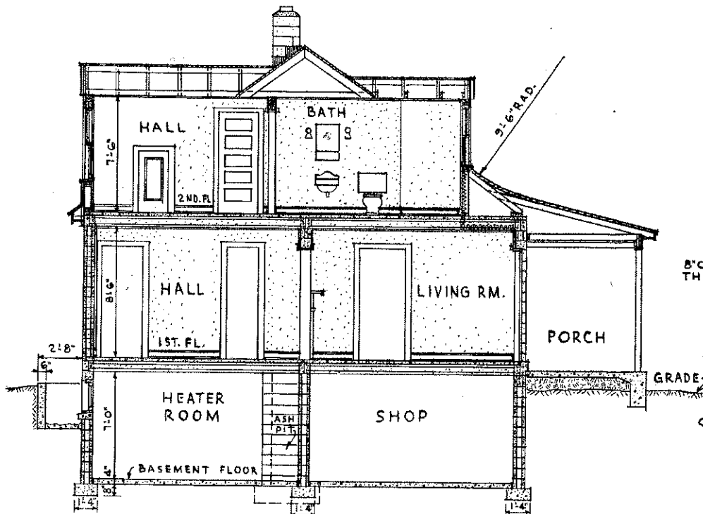
CROSS SECTION SCALE \frac{1}{4}'' = 1'-0''
