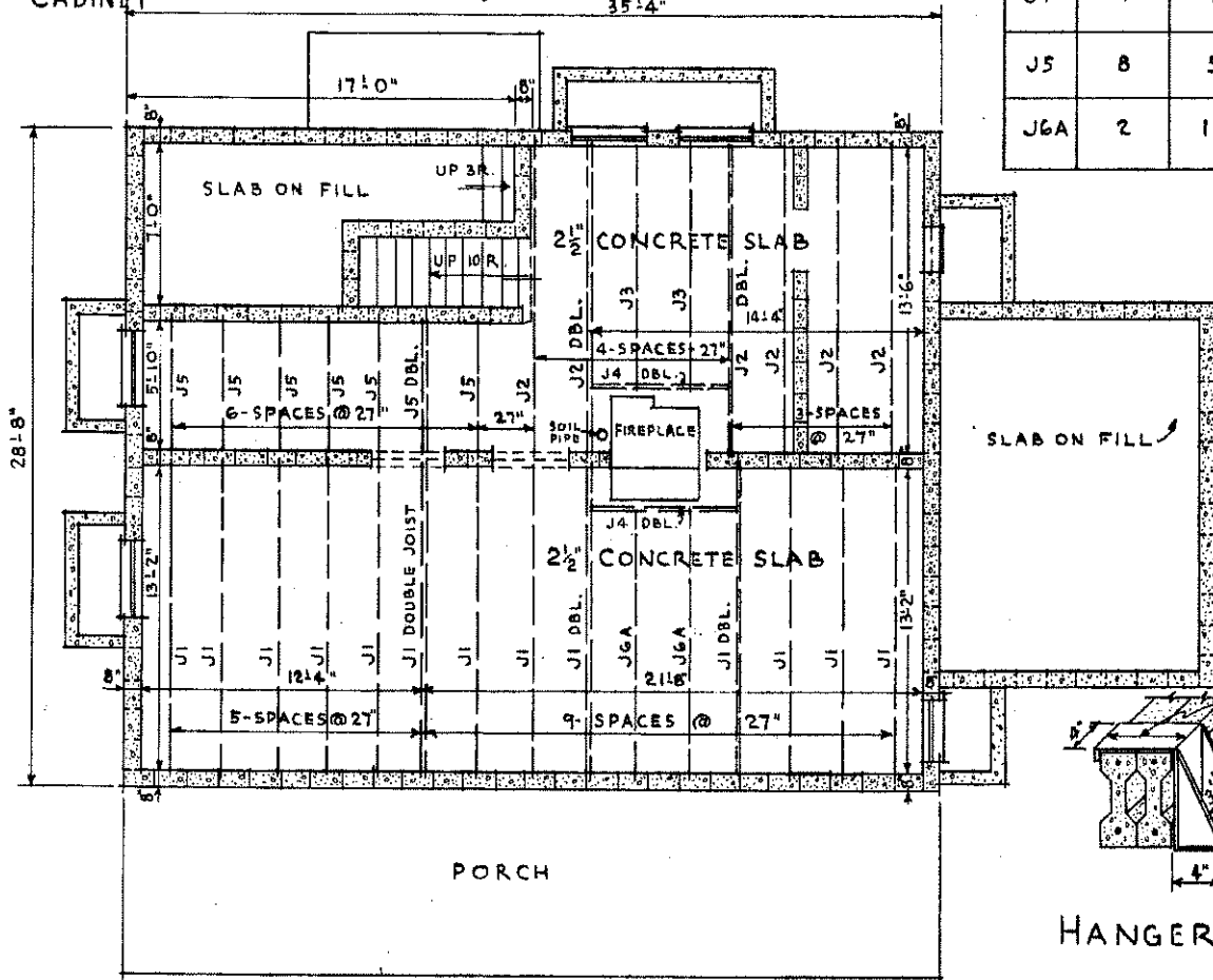
FRAMING FOR FIRST FLOOR CONCRETE JOISTS SCALE 1/4" = 1'-0"
