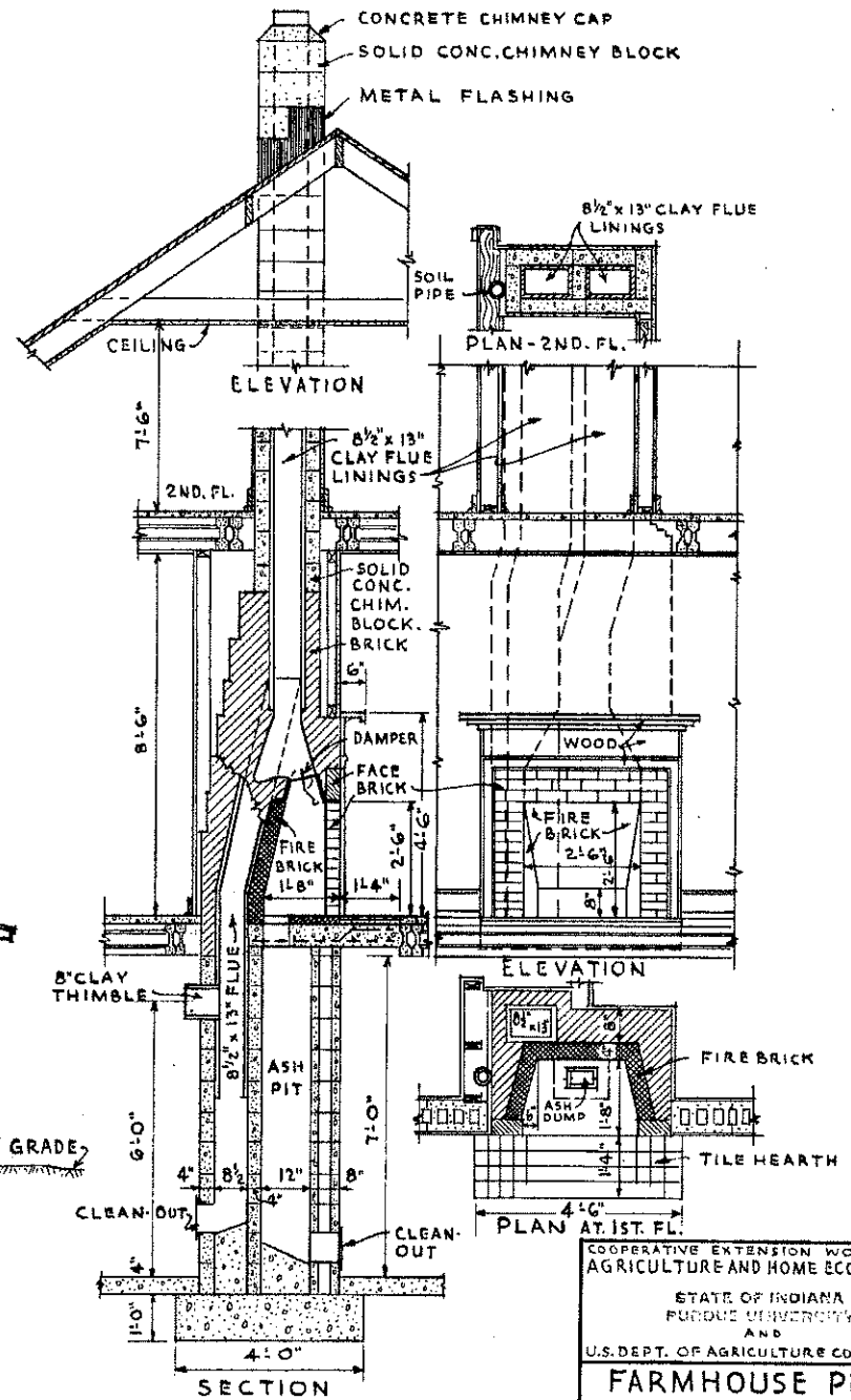
DETAILS OF FIREPLACE SCALE \frac{1}{2}'' = 1'-0''
