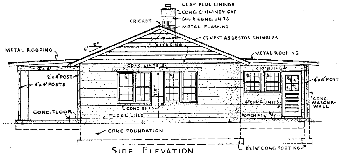
SIDE ELEVATION SCALE 1/4" = 1'-0"
