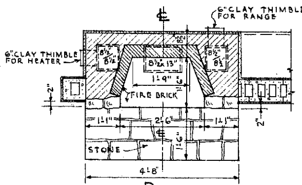
DETAILS OF FIRE PLACE SCALE \frac{3}{4} " = 1'-0"
