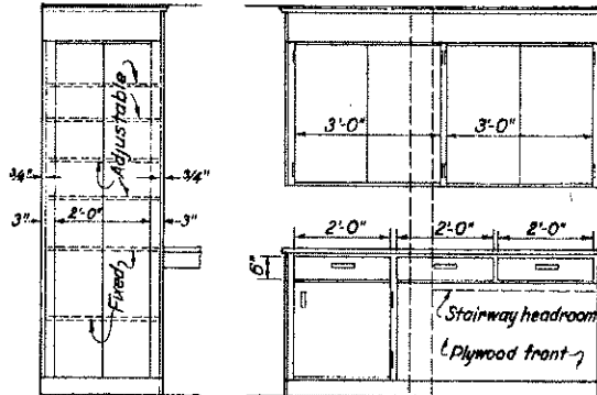
KITCHEN ELEVATIONS* C
