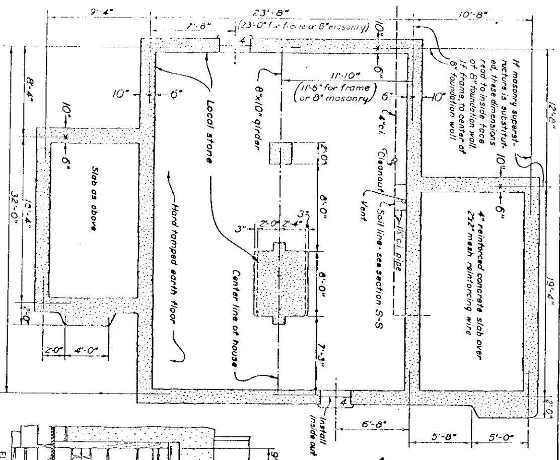
FOUNDATION PLAN
