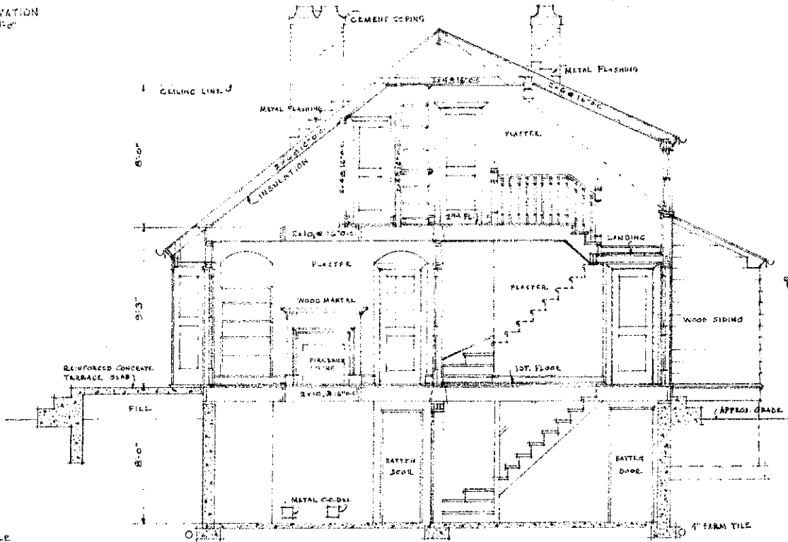
CROSS SECTION Scale \frac{1}{4}'' = 1'-0''
