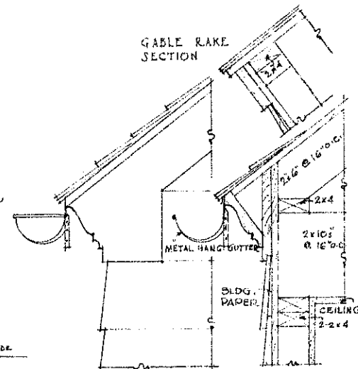
GABLE RAKE SECTION GABLE RETURN SECTION MAIN CORNICE DETAILS Scale \frac{1}{2}'' = 1'-0''
