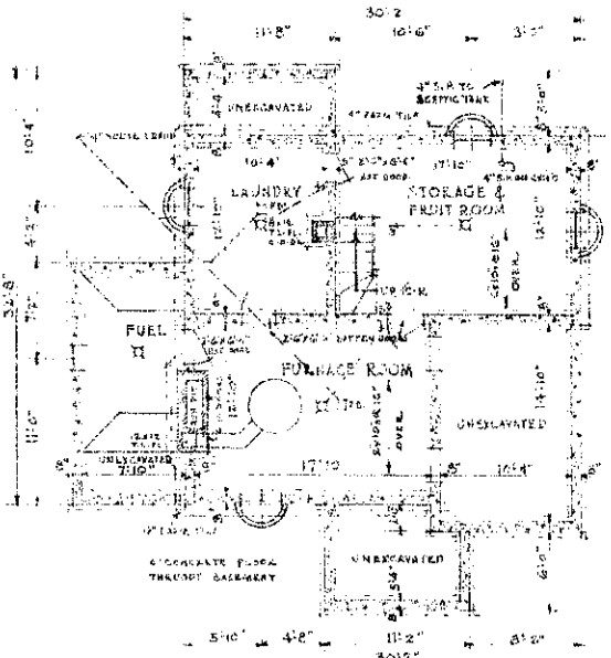
BASEMENT PLAN Scale 3/8" = 1'-0"
