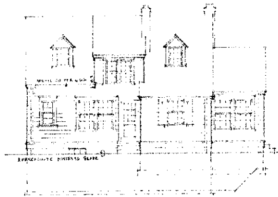
REAR ELEVATION Scale \frac{1}{8}'' = 1'-0''
