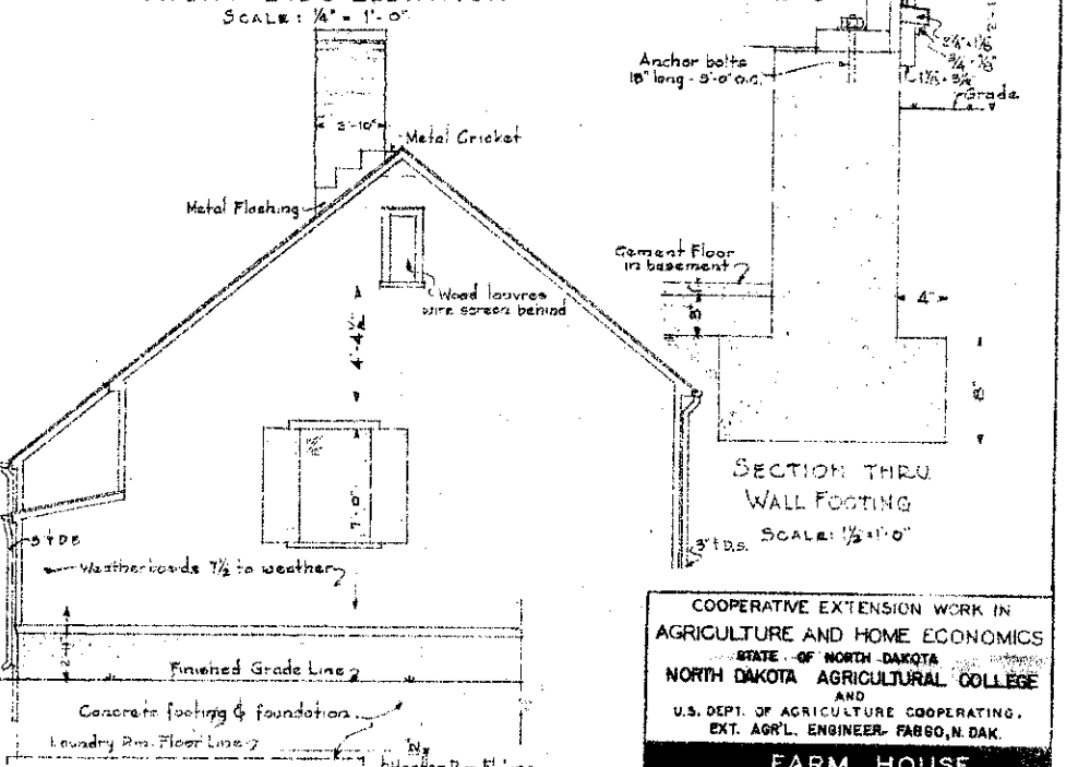
LEFT SIDE ELEVATION SCALE: 1/4" = 1'-0"
