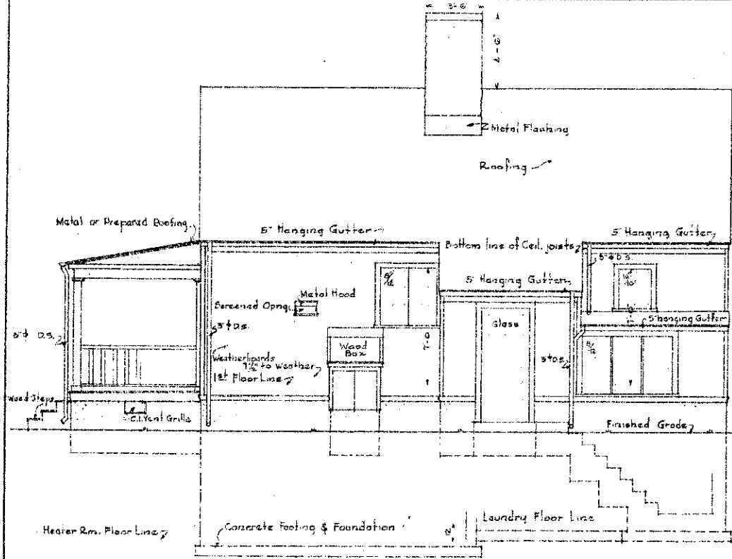
REAR ELEVATION SCALE: 1/4" = 1'-0"
