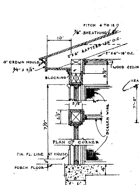
DETAILS OF PORCH CONSTRUCTION SCALE - 1" = 1'-0"
