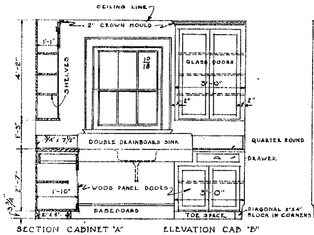
ELEVATIONS OF KITCHEN SHOWING CABINET DETAILS SCALE - 1/2" = 1'-0"
