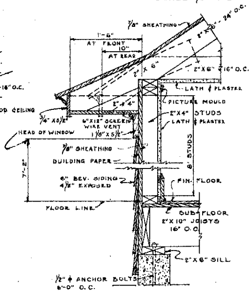
TYPICAL WALL SECTION SCALE - 1" = 1'-0"
