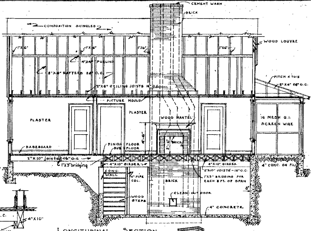
LONGITUDINAL SECTION SCALE 1/4" = 1'-0"
