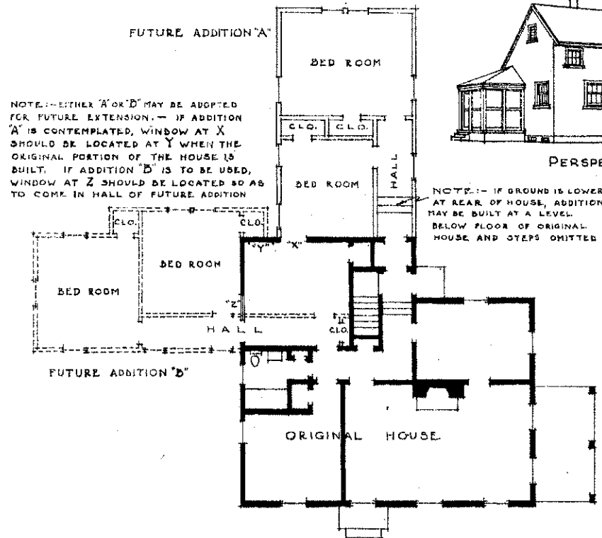
PLAN SHOWING SUGGESTIONS FOR FUTURE ADDITIONS SCALE - 1/8" = 1'-0"
