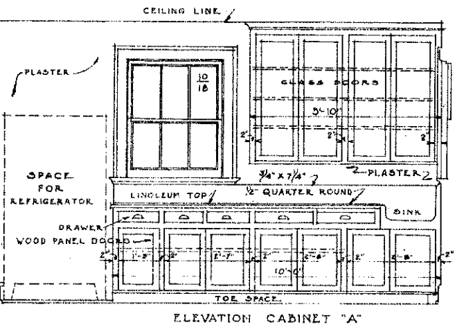
ELEVATIONS OF KITCHEN SHOWING CABINET DETAILS SCALE - 1/2" = 1'-0"
