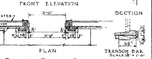
DETAILS - FRONT ENTRANCE DOOR SCALE 1/2" = 1'-0"
