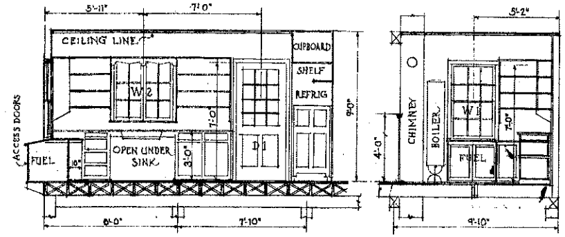
SECTIONS THRU KITCHEN
