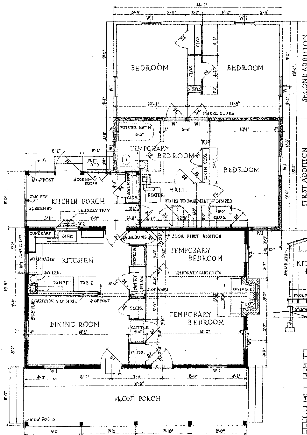
ORIGINAL FLOOR PLAN SCALE 1/4"=1'-0"
