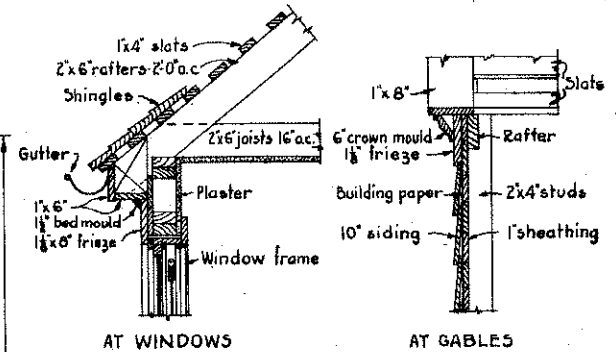
CORNICE DETAILS Scale 3/4" = 1'-0"
