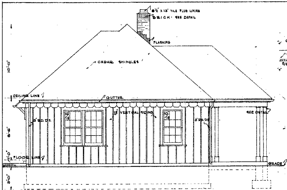
DRIVEWAY ELEVATION SCALE 1/4"=1'-0"
