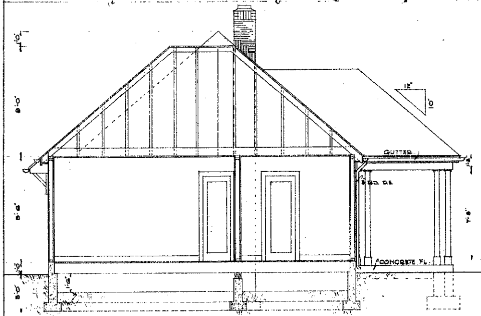
SECTION THRU LIVING RM. DINING RM. & KITCHEN SCALE 1/4"=1'-0"
