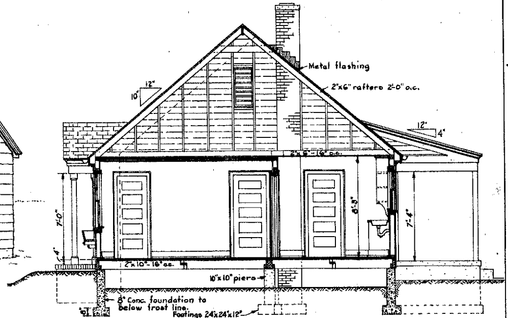
SECTION "A-A" Scale 1/4" = 1'-0"
