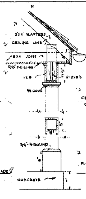
PORCH DETAIL SCALE 1/2"=1'-0"
