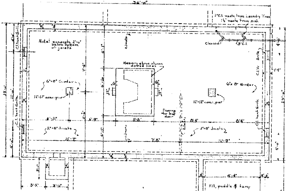
FOUNDATION PLAN scale 1/4" = 1'-0"
