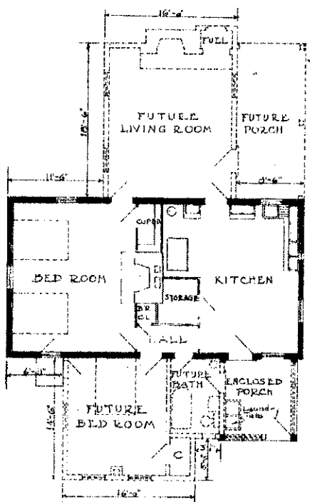
PLAN Showing Arrangement with Future Additions scale 1/8" = 1'-0"
