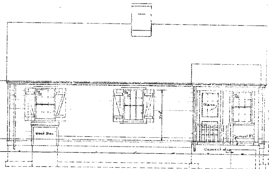
LEFT SIDE ELEVATION scale \frac{1}{4}'' = 1'-0''
