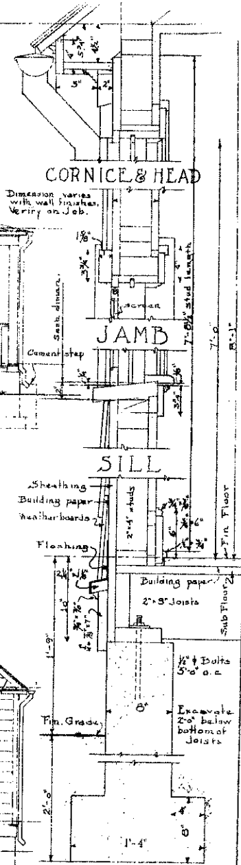
FOOTING WALL SECTION scale \frac{1}{2}'' = 1'-0''
