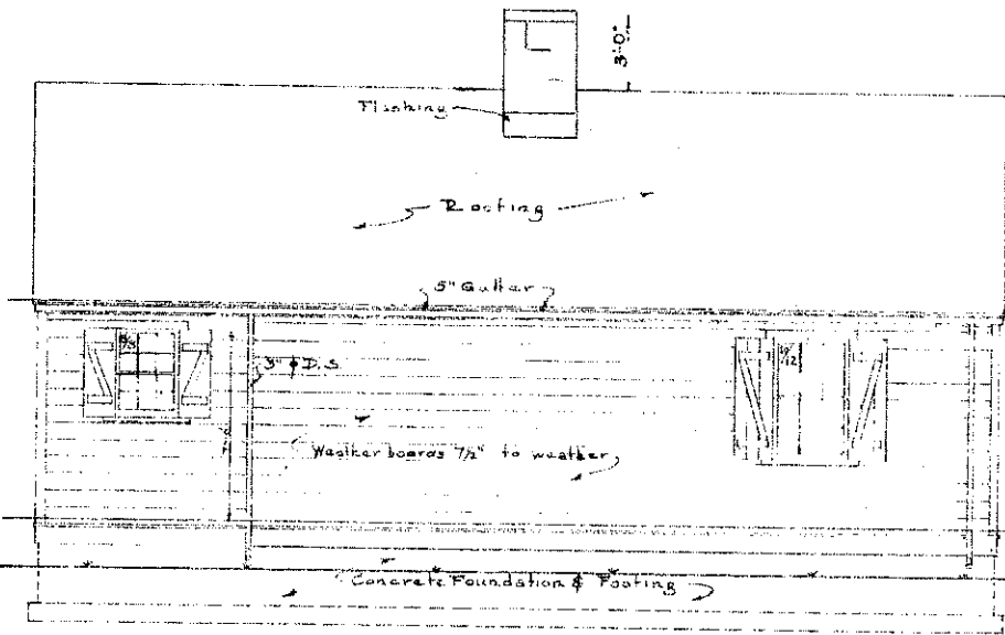
RIGHT SIDE ELEVATION scale \frac{1}{4}'' = 1'-0''
