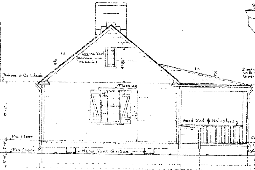
REAR ELEVATION scale \frac{1}{4}'' = 1'-0''
