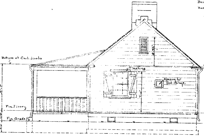
FRONT ELEVATION scale \frac{1}{2}'' = 1'-0''
