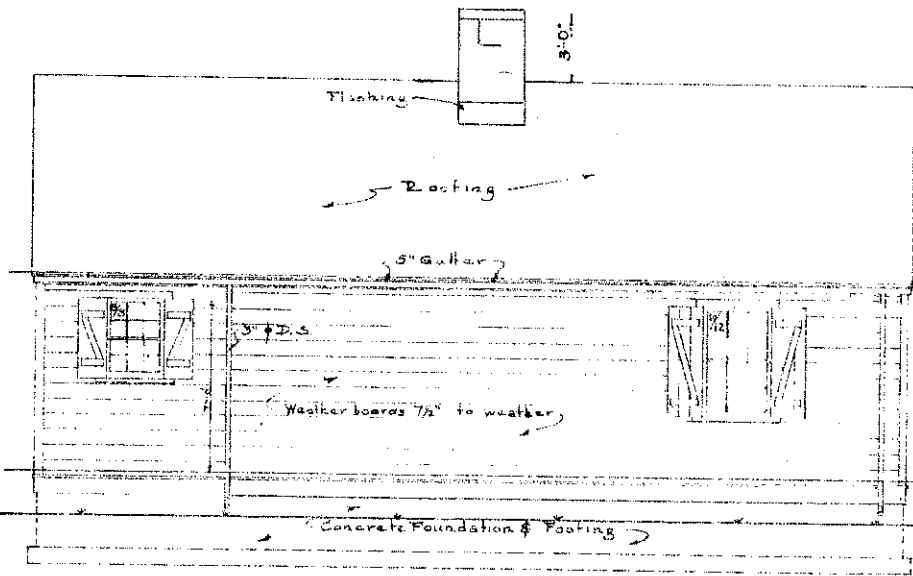
RIGHT SIDE ELEVATION scale \frac{1}{4}'' = 1'-0''
