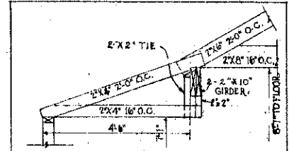
DETAIL OF KITCHEN CEILING CONSTRUCTION
