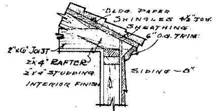
SECTION, THRU CORNICE SCALE 1/2" = 1'-0"
