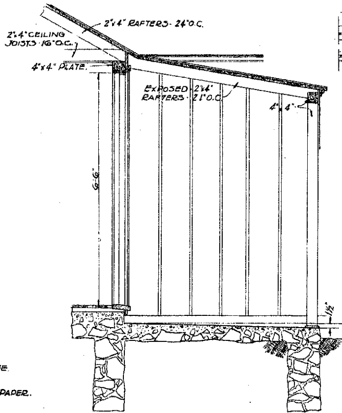
SECTION THRU PORCH
