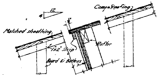
GABLE TRIM Scale 1/2" = 1'-0"
