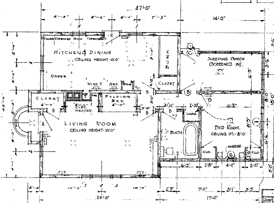
ORIGINAL HOUSE. FLOOR PLAN NO. 11A (PLAN 1111) SCALE 1/8" = 1'-0" 1ST ADDITION
