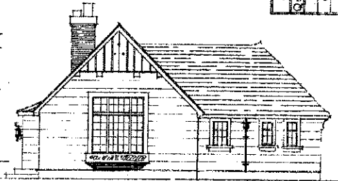
ELEVATION SCALE 1/4" = 1'-0"
