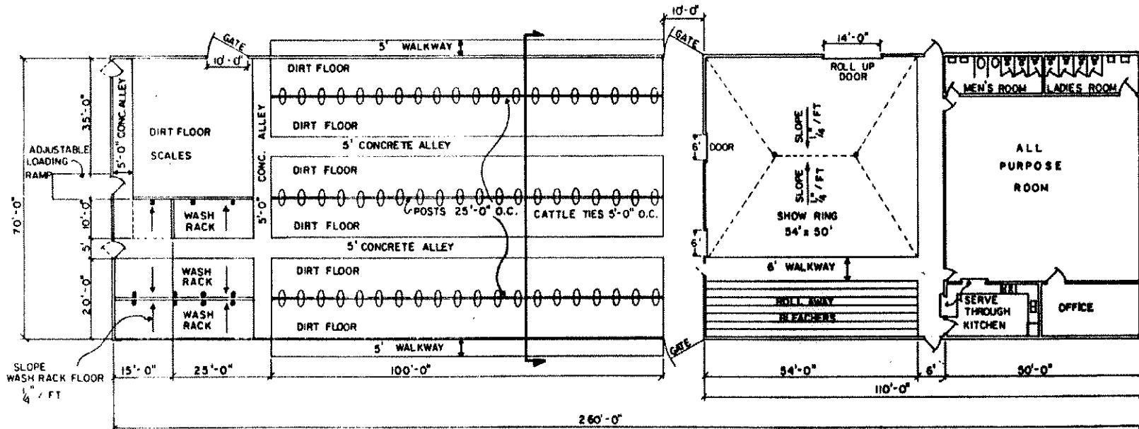
FLOOR PLAN
