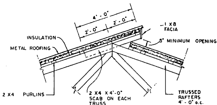
RIDGE VENT DETAIL
