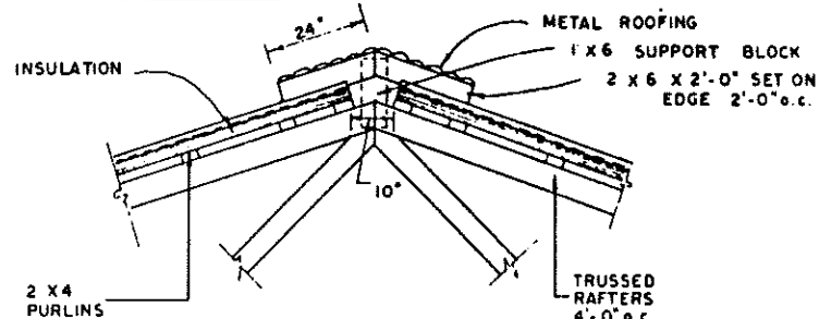
ALTERNATE RIDGE VENT
