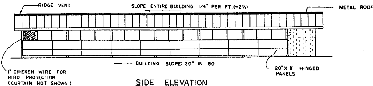
SIDE ELEVATION
