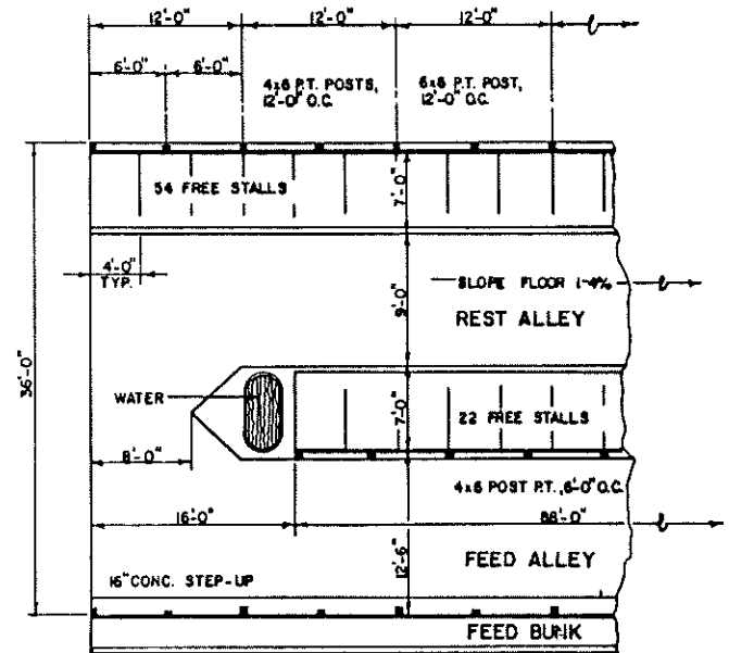
TYPICAL DETAIL
