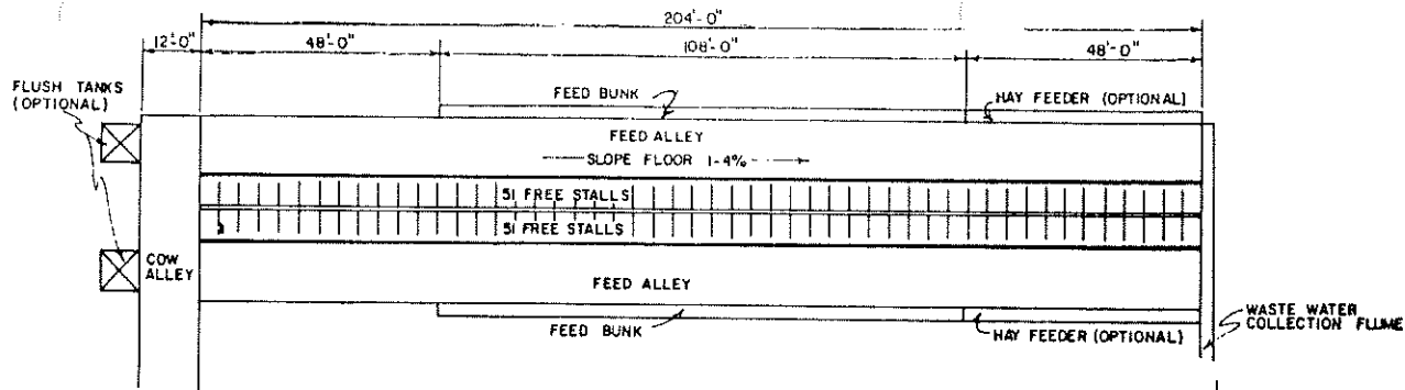
FLOOR PLAN
