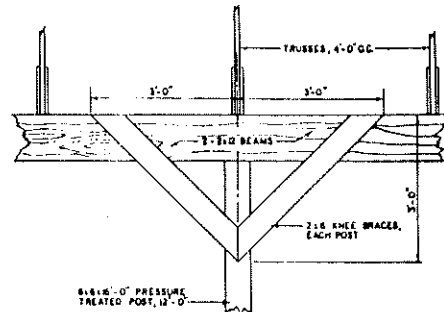
KNEE BRACE DETAIL (FOR ALL LAYOUTS)
