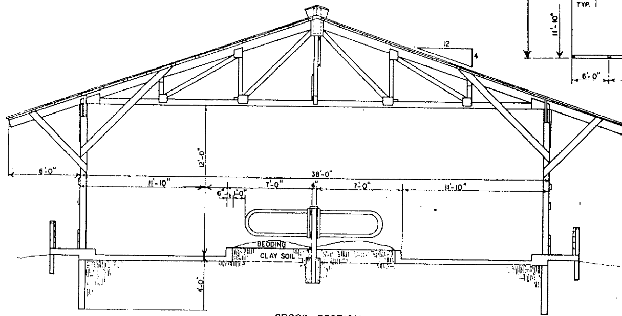
CROSS SECTION
