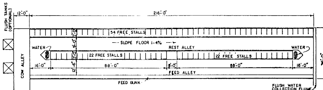
FLOOR PLAN
