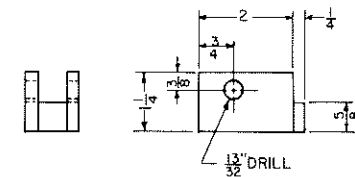
HINGE DETAILS
