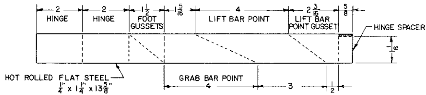
STRAP STEEL CUTTING DIAGRAM
