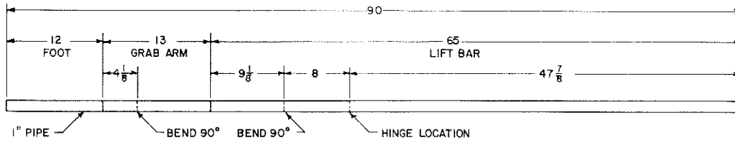
BLACK IRON PIPE CUTTING DIAGRAM
