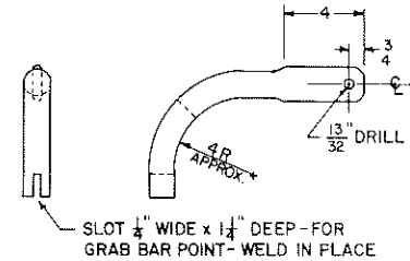
GRAB BAR DETAILS
