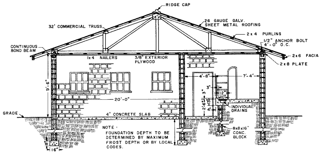
SECTION "A-A" SCALE 12' 0' 1' 2' 3' 4' 5' 6' 7' 8'
