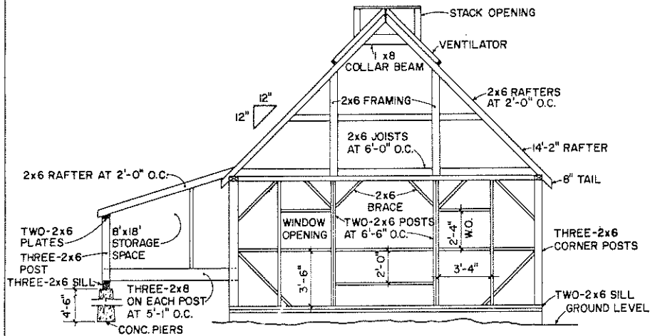
NORTH END FRAMING
