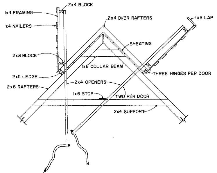
SECTION THROUGH VENTILATOR
