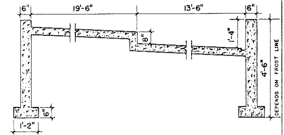
SECTION THROUGH FOUNDATION SCALE: 1/8" = 1'-0"
