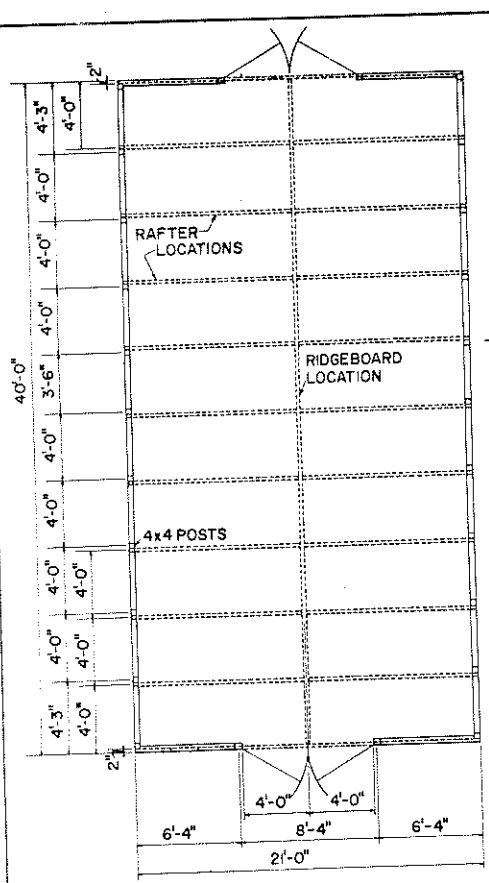
FLOOR PLAN SCALE: 1/2" = 1'-0"
