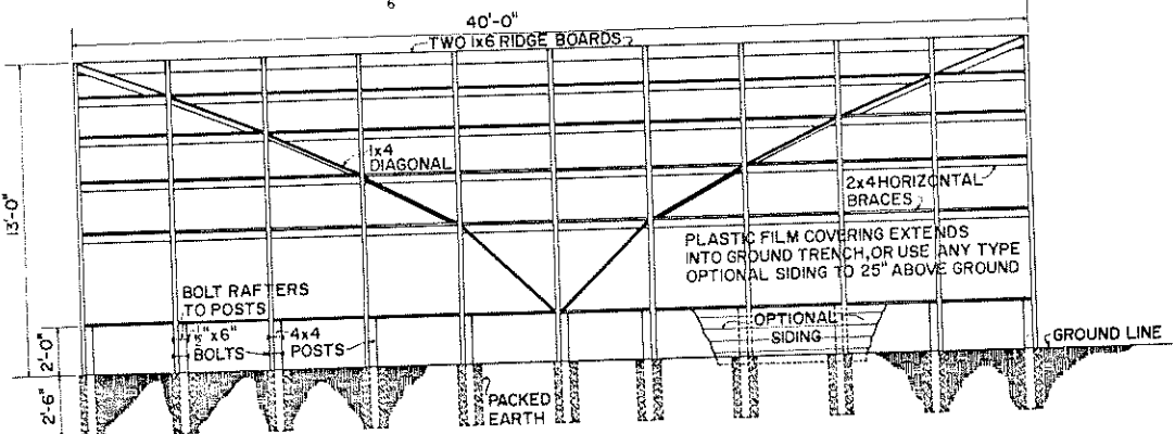
SIDE VIEW OF FRAMING
