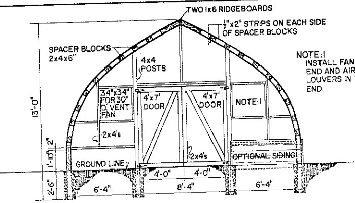
END VIEW OF FRAMING
