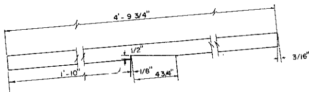
RAFTER DETAIL (NOT TO SCALE)
