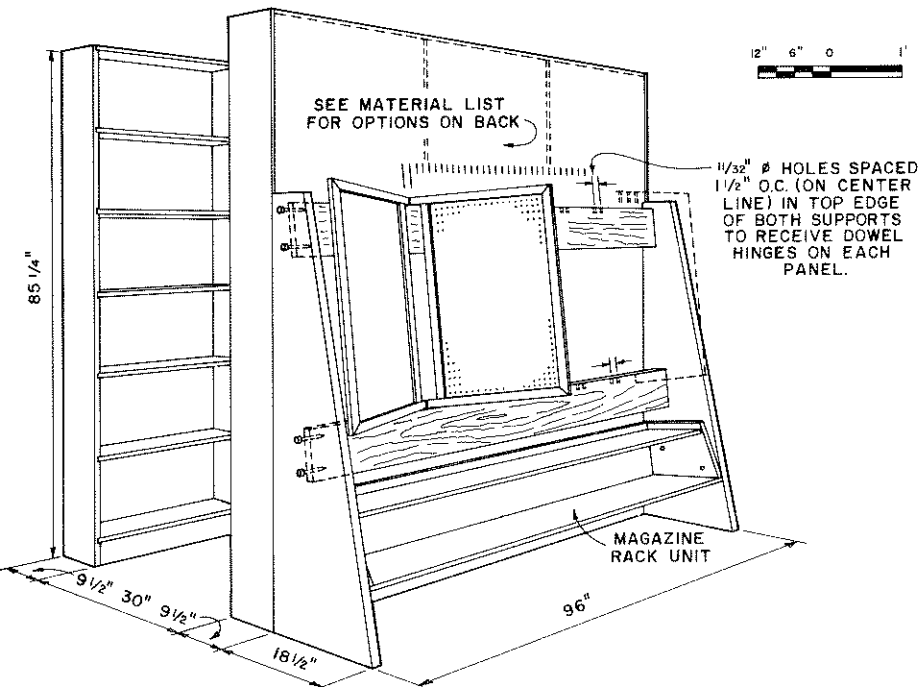
OVERALL VIEW SHOWING SPACE REQUIREMENTS NO SCALE
